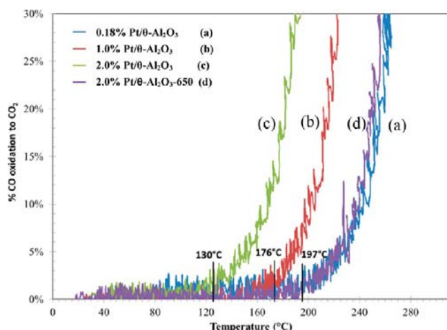
Figure 5. CO conversion to CO 2 for the Pt/ \theta -Al 2 O 3 samples.
