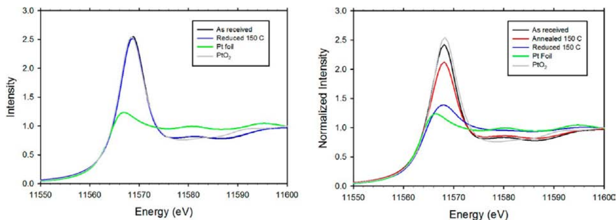
Figure 2. Pt L III -edge XANES for 0.18% Pt on \theta -Al 2 O 3 (left) and 1.0% Pt on \theta -Al 2 O 3 (right).
