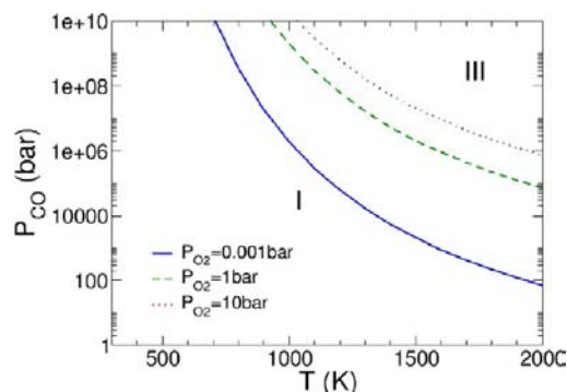
Figure 10. Phase diagram of configurations I and III (see Scheme 2) as a function of temperature ( T ) and CO gas pressure ( P_{CO} ) was obtained using the first-principles thermodynamics approach. Each line defines the phase boundary between I and III. Above the phase boundary, III is relatively more stable than I for a given oxygen pressure ( P_{O_2} ).
