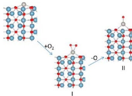
Scheme 1. Interaction of Oxygen with Pt/ \theta -Al 2 O 3
