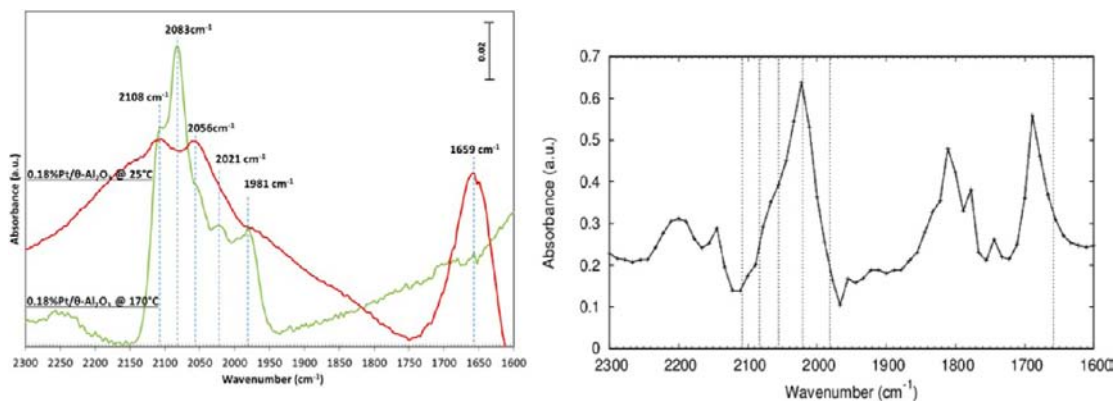
Figure 12. DRIFTS spectra of CO adsorption on 0.18% Pt/ \theta -Al 2 O 3 at 25 and 170 °C (left), and calculated vibrational spectrum of III. Vertical lines correspond to the vertical lines in the observed spectrum shown on the left.
