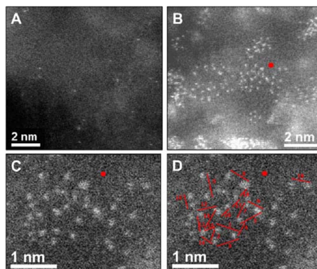
Figure 1. ACEM HAADF-STEM images 0.18% Pt/ \theta -Al 2 O 3 (A and B, respectively). (C and D) Identical enlargements of a portion of B with the red dot used as a reference point. Numbers in image D correspond to various observed Pt–Pt distances summarized in Table 2.
