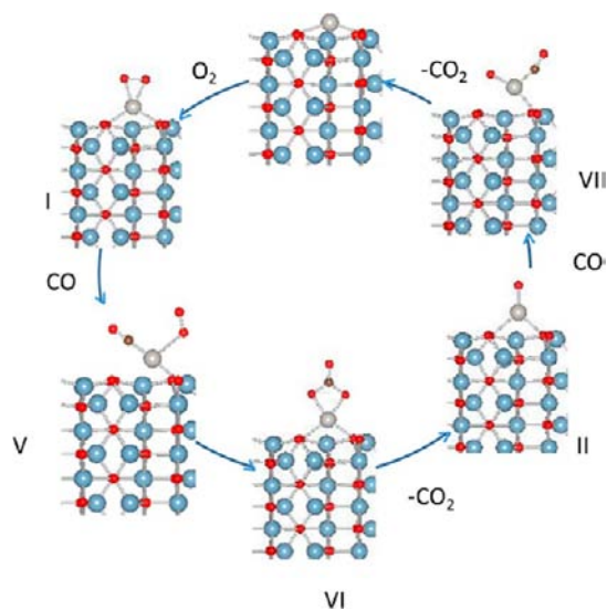
Scheme 3. Pathway for CO Oxidation on Single Pt Atoms Supported on the (010) Surface of \theta -Al 2 O 3
